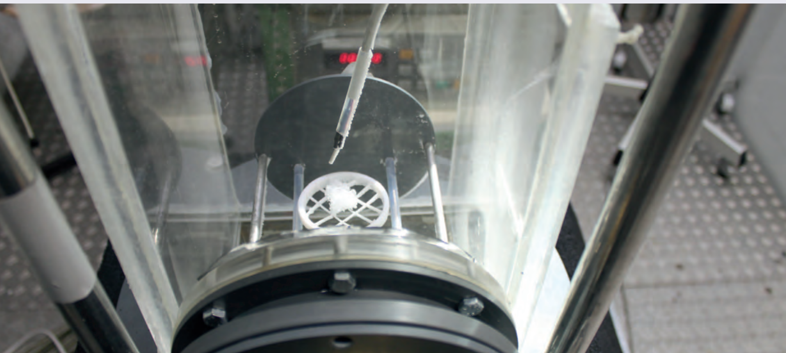
Figure 1: Shown is the insulated box which is fixed at the wall of the experimental section of the wind tunnel. The rime collector is exposed in the center of the section and, thus, in the cloud of supercooled droplets. The air flow enters from below the picture.
