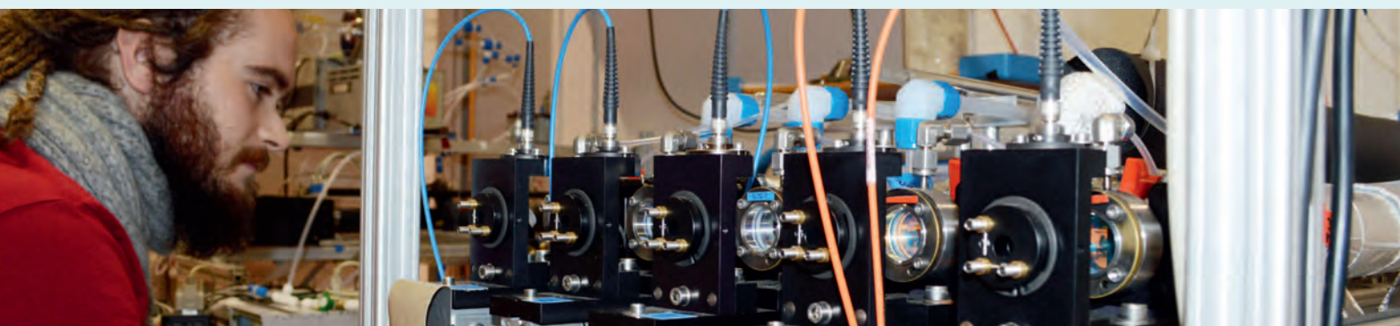
Figure 1: Cavity-ring-down spectrometer.
