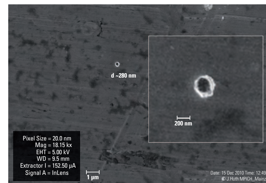
Figure 2: SEM image of a 280 nm-sized impact crater on an Al foil target from NASA’s Stardust mission. The impactor was likely an interstellar Mg-Fe-rich silicate grain.
