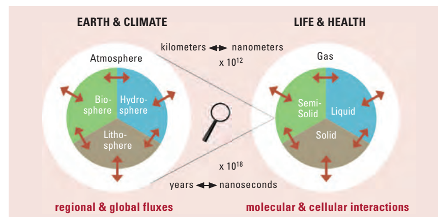
Figure 2: Multiphase processes on molecular to global scales affecting the Earth System, climate, life, and public health.
