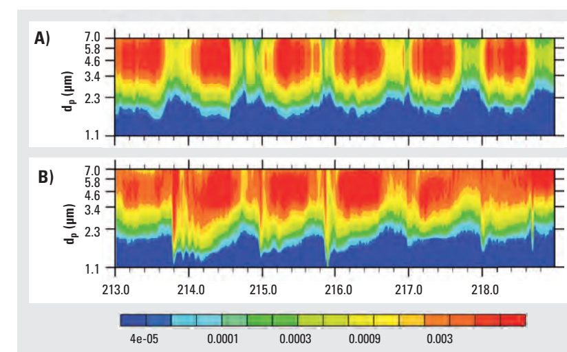
Figure 3: Mass size distributions of PBAP from model (A) and observation (B), Color bar: \text{dM/dlog}d_p .
