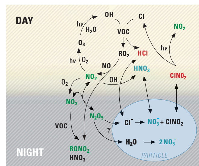
Figure 2: By influencing daytime \text{NO}_x and also via the formation of Cl atoms, heterogeneous chemistry during the night can have a profound impact on daytime photochemical processes.
