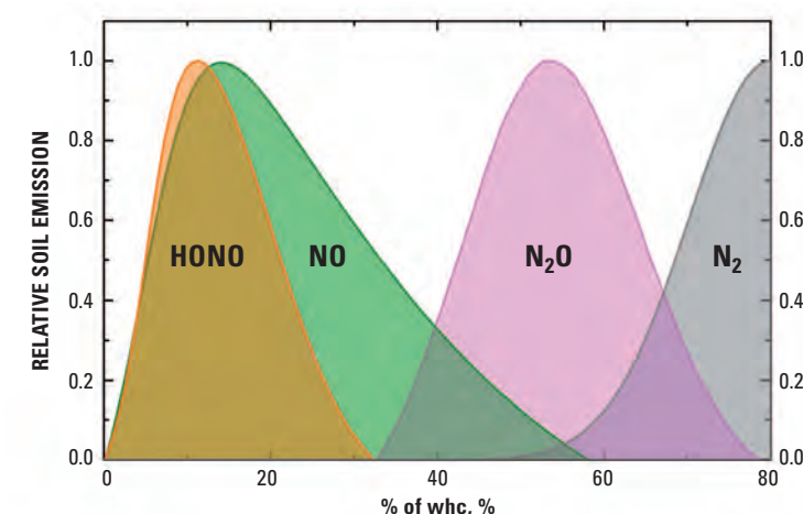
Figure 2: Conceptual model of emissions of reactive nitrogen from soils. From Oswald et al. (2013).
