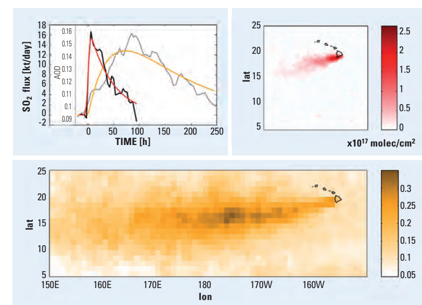
Figure 2: Top left: Temporal evolution of line densities of \text{SO}_2 (black: measured; red: fitted) and averaged AOD (grey: measured; orange: fitted); Top right: Monthly mean distribution of the \text{SO}_2 VCD; Bottom: Monthly mean distribution of the AOD (all results for August 2008).
