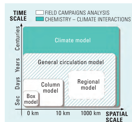
Figure 2: A hierarchy of connected models can be used to study atmospheric processes from local to global scales.
