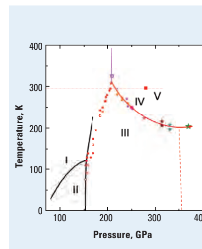
Figure 1: Phase diagram of hydrogen. Black lines are boundaries between phases I, II, and III established in previous works (Mao and Hemley, 1994). Our experimental data established borders of new phases.
