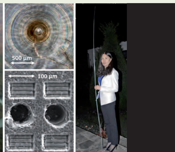
Figure 2: Giant spicule from the deep sea sponge Monorhaphis chuni (right). Lamellar organization of the spicule and laser craters (rectangular scans and round spots for Si isotope and Ge concentration measurements, respectively) (left).
