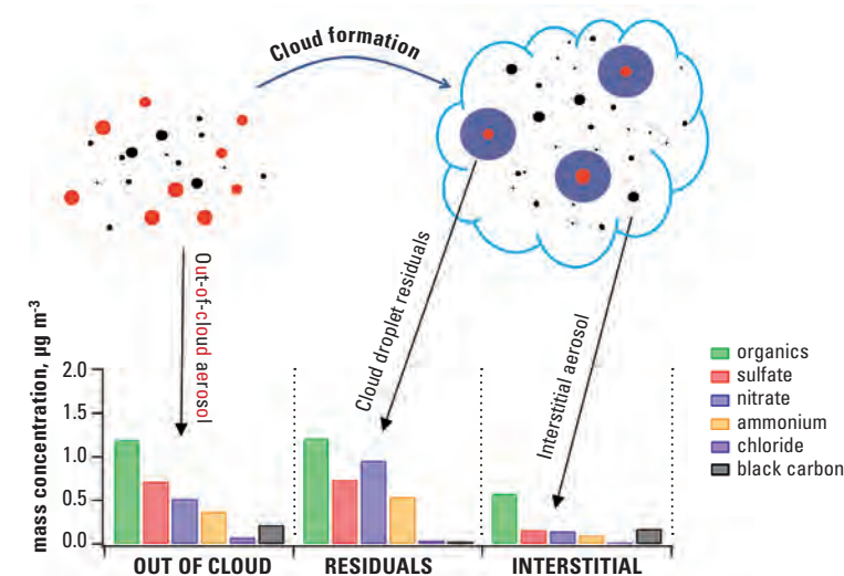
Figure 2: Aerosol composition before and during cloud occurrence. The absolute amount of nitrate increases in the cloud due to uptake of nitric acid from the gas phase by the cloud droplets. Black carbon remains mainly in the unactivated interstitial aerosol.
