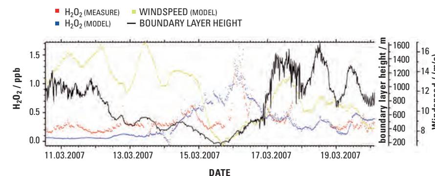
Figure 2: H_2O_2 observations and EMAC simulations in the marine boundary layer over the southern Atlantic Ocean. The model tends to underestimate H_2O_2 at high wind speeds during the first half of the campaign, but agrees well at wind speeds below 10 m/s.
