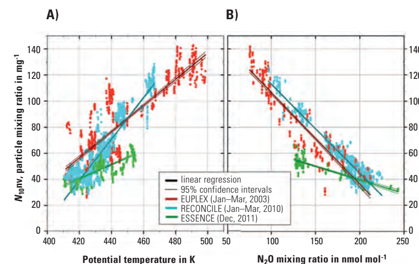
Figure 2: Dependence of the mixing ratio of non-volatile particles N_{10nv} as function of potential temperature (Panel a) and of N 2 O mixing ratio (Panel b), linear regressions with 95% confidence intervals are shown. Results from measurements within the vortex are shown for the three Arctic missions: EUPLEX (2003), RECONCILE (2010) and ESSence (2011).
