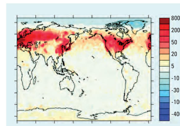
Figure 3: EMAC model calculated relative change in OH (in %) near the surface in December, indicating the relative difference between the standard and the parameterized HONO representation for the month January.
