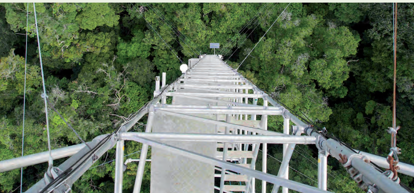
Figure 1: Working 80 m above ground level and 40 m above the crowns of the trees of the Amazonian rain forest.
