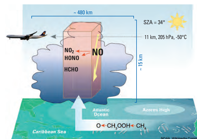
Figure 2: Schematic of the main features of the event near the island of Guadalupe. The multiple reflection of photons inside the cloud enhanced the detection limit for HCHO and HONO by DOAS remote sensing. Both trace gases were more abundant. HONO due to the production of NO x by lightning. HCHO due to convection giving an input of surface air with higher HCHO and precursor levels.
