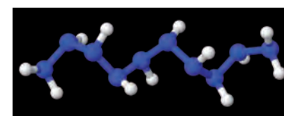
Figure 3: Ball and stick representation of \text{N}_{10}\text{H}_{12} , illustrating the low-energy spiral backbone structure.
