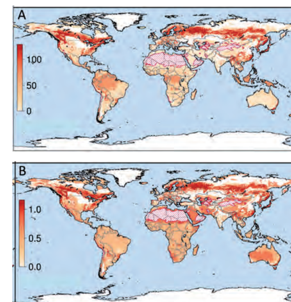
Figure 2: Global maps of \text{N}_2 fixation (A) and \text{CO}_2 uptake (B) by cryptogamic covers. The flux units are \text{g m}^{-2} \text{ a}^{-1} . White areas indicate ecosystems for which no data are available; hashed areas are excluded from calculations due to low precipitation amounts (adapted from Elbert et al. 2012).
