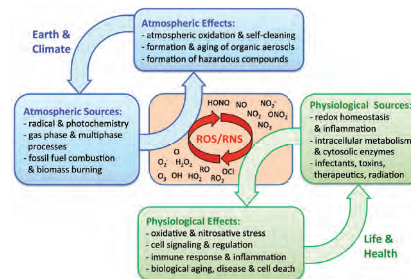
Figure 2: Reactive oxygen & nitrogen species (ROS, RNS): Sources, effects and interactions at the interface of atmospheric and physiological chemistry, with feedback loops involving the Earth System, climate, life, and health (adapted from Shiraiwa et al. 2012).
