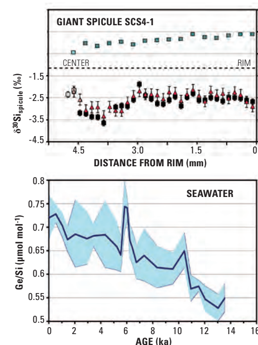
Figure 3: (Top) \delta^{30}\text{Si} values and Ge abundances obtained from microanalyses of a cross section of the giant spicule SCS4-1 from the South China Sea. Data from this and other spicules are used to determine seawater Ge and Si concentrations in the deep-sea environment in the last 14 ka. (Bottom) Ge/Si ratios have slightly increased during the Holocene (from about 10.5 ka B.P. to present) with a possible maximum at about 5 – 6 ka B.P., which may be related to the Holocene climatic optimum. Low Ge/Si values (10.5 – 13.5 ka B.P.) correspond to the Younger Dryas cold period.
