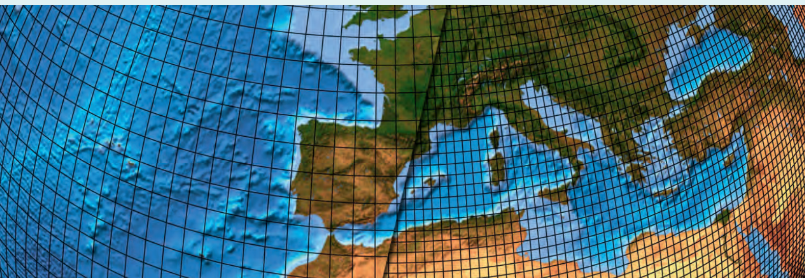
Figure 1: Resolution grid for a typical global numerical model.
