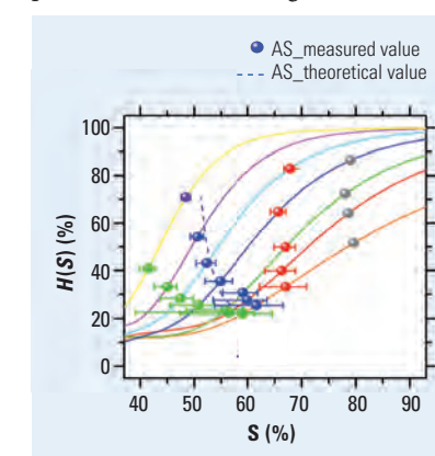
Figure 3: Supersaturations determined for particles of mobility diameter 2.5 nm sodium chloride (green), ammonium sulfate (AS, blue), sucrose (red) and tungsten oxide (gray) aerosols. Solid lines indicate different cumulative effective supersaturation distributions.
