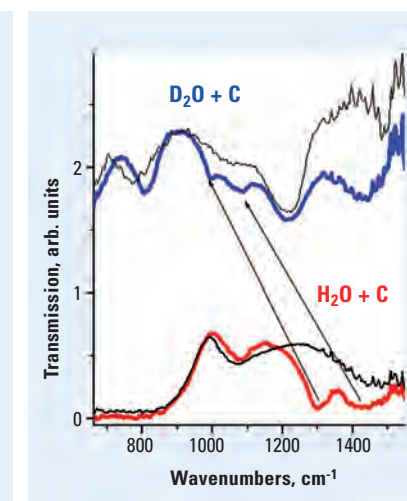
Figure 2: Synthesis of hydrocarbons from carbon and water at 3 GPa and 1000°C. Infrared transmission spectra. The peak at 1310\text{ cm}^{-1} is characteristic for methane, others to higher hydrocarbons.
