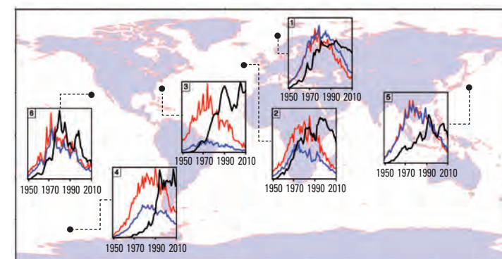
Figure 2: Trends of PCB153 depositions (red, \text{ng m}^{-2} \text{a}^{-1} ), surface layer (0–100 m; blue) and deep water layer (depths at locations 1–6: 500–1,000 m, 700–1,200 m, 1,000–1,500 m, 1,000–1,500 m, 700–1,200 m, and 200–500 m, respectively; black) concentrations ( \text{ng m}^{-3} ) at 6 locations in the world oceans.
