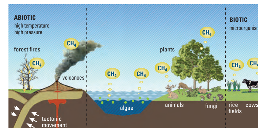
Figure 2: Sources of methane in the environment. For decades scientists only knew forest fires, fossil fuel use and geological processes such as volcano outgassing as abiotic methane sources. Microorganisms were considered as the only biotic source to produce methane without oxygen. We have found that aerobic organisms such as plants, fungi, lichens and algae also produce methane. Whether this is biotic, i.e. catalyzed by enzymes, or abiotic is currently being investigated.
