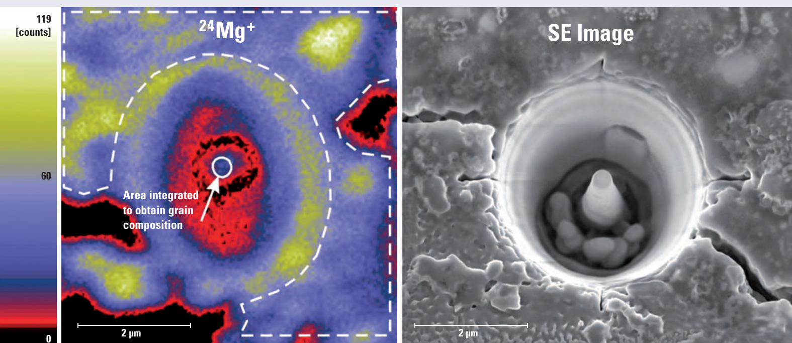
Figure 1: Magnesium-24 isotope image acquired with the NanoSIMS ion probe (left) after FIB preparation (right) of a stardust silicate from the Acfer 094 meteorite. The stardust grain sits on top of the tip prepared by FIB.
