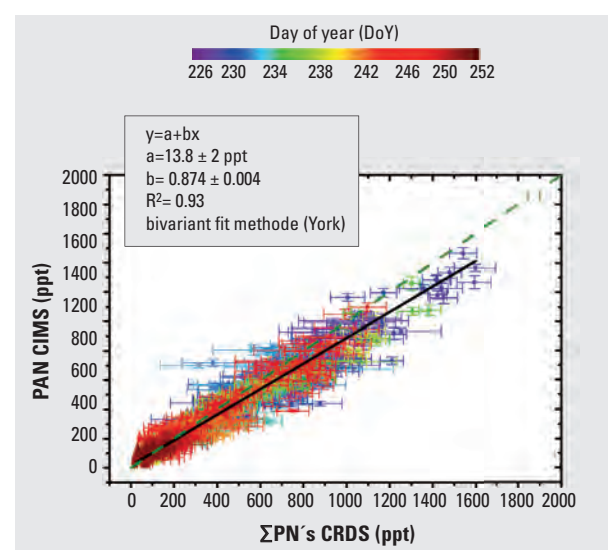
Figure 3: PAN (measured by chemical ionization mass spectrometry) is about 80–90% of total peroxy nitrates ( \Sigma[\text{PNs}] ).
