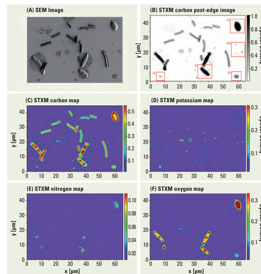
Figure 2: Microscopic images of Amazonian wet season aerosol particles. (A) SEM images of representative region. (B) STXM carbon post-edge image (293 eV) and (C-F) STXM elemental maps of same region.
