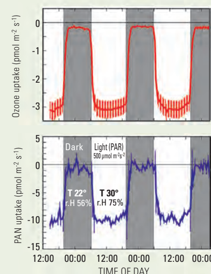
Figure 2: Dynamics of trace gas exchange between soils (COS), plants (PAN, \text{O}_3 ; Quercus ilex) and the atmosphere measured with soil or plant enclosures under controlled conditions. Error bars represent errors according to the Gaussian propagation method.
