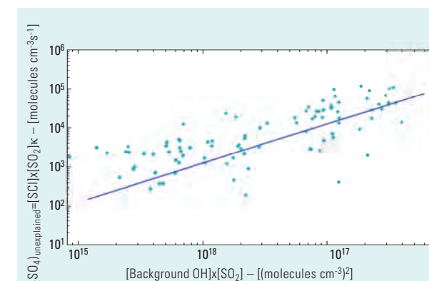
Figure 1: Correlation between the OH generated from unimolecular decomposition of an unknown species (OH excluded) in our instrument and the production rate of \text{H}_2\text{SO}_4 over the Boreal forest.
