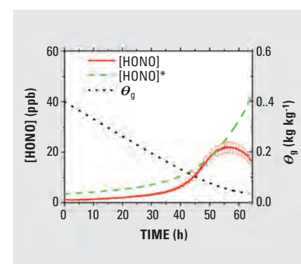
Figure 2: Chamber measurements of HONO emission from soil. [HONO] represents the measured gas phase HONO concentration (red solid line) and \theta_g represents the gravimetric soil water content (black dots) (adapted from Su et al. 2011).
