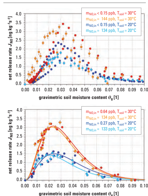
Figure 2: Results of individual NO net release rate ( J_{\text{NO}} ) measurements performed on 12 sub-samples of a desert soil from Mongolia. Measurements with the previous (before 2013) laboratory chamber system (top) and the present day system (bottom). Two (bottom) and three (top) replicates have been measured for each of the four measurement conditions indicated by the four different colors of shown data points.
