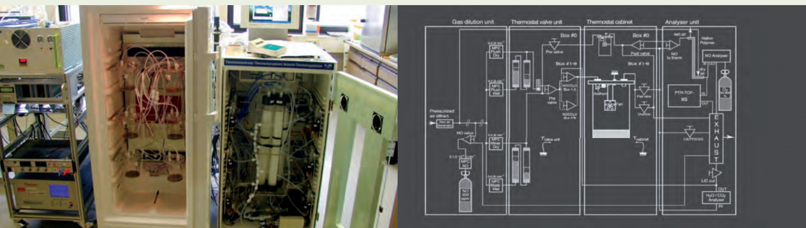
Figure 1: Fully automated incubation system for simultaneous fumigation of six soil samples under prescribed conditions of soil moisture, soil temperature and NO concentration: humidifiers, mass flow controls, and valve manifolds, dynamic soil chambers and soil sensors (left). Schematic setup of the improved laboratory incubation system (right).
