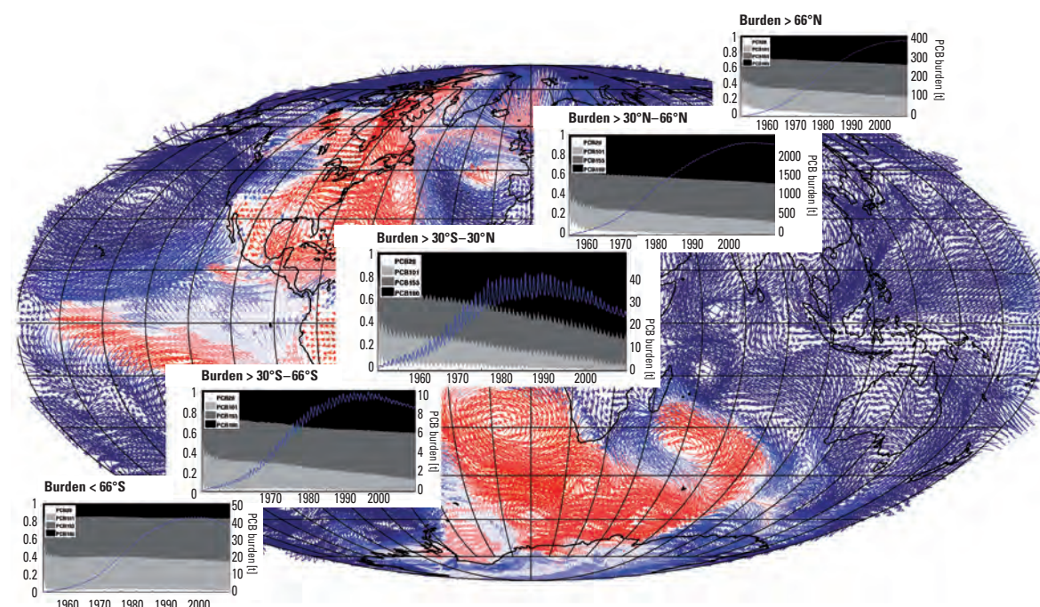
Figure 1: Global fractionation of PCB congeners with 3–7 chlorine atoms 1950–2010.
