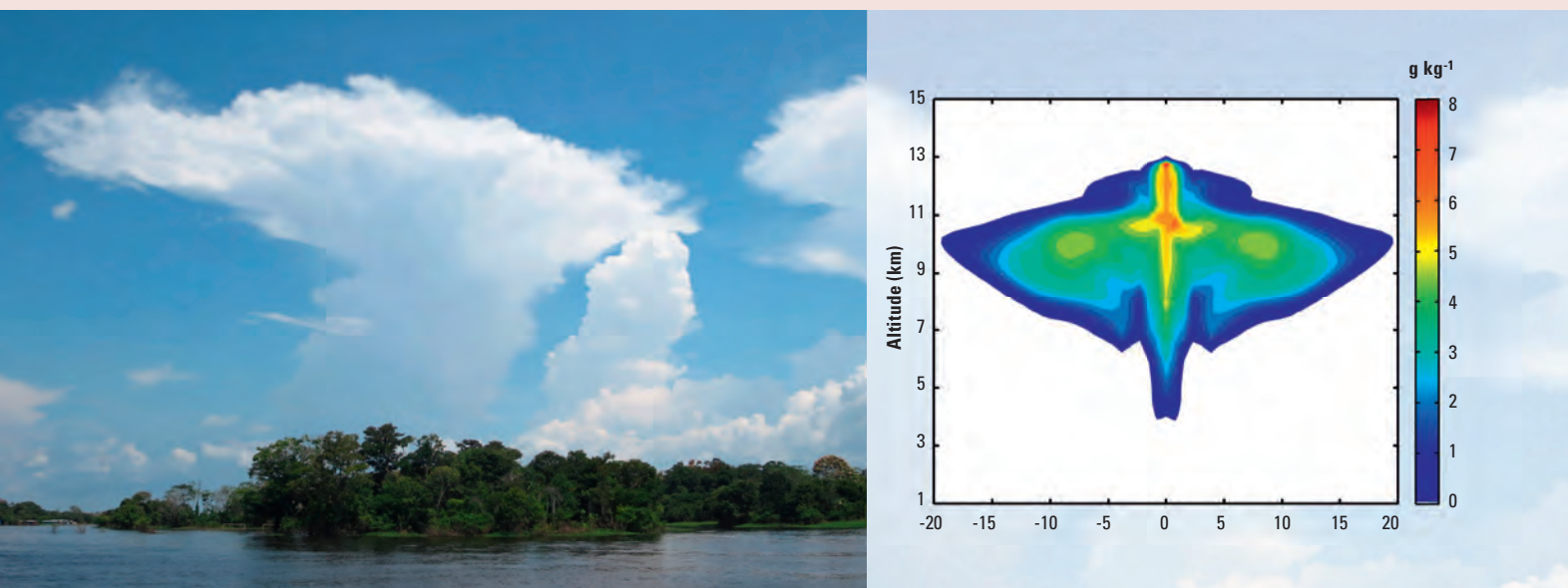
Figure 1: Convective clouds as observed over the Amazon (left) and simulated with a numerical model (right).
