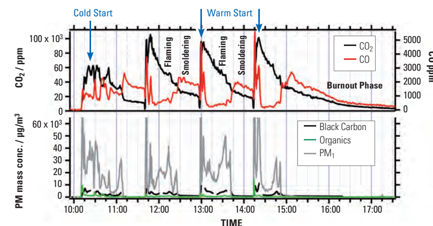
Figure 2: Temporal trends of concentrations of trace gases (CO, CO 2 ) and particle components (PM 1 , black carbon, particulate organics) during four consecutive wood burning experiments.
