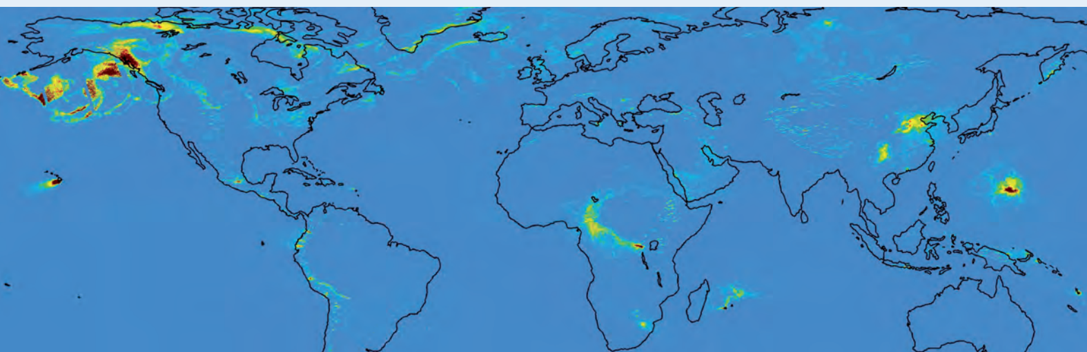
Figure 1: Composition of monthly averaged \text{SO}_2 vertical column densities as seen by the OMI satellite instrument. Besides anthropogenic and passively degassing volcanic sources, the picture shows volcanic plumes during major eruptions of Anatahan (2005), Nyamuragira (2006), Piton de la Fournaise (2007) and Kasatochi (2008).
