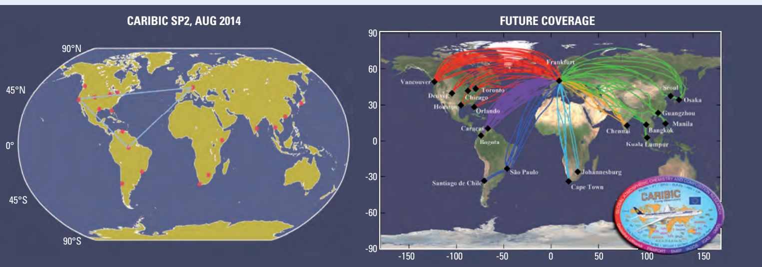
Figure 1: Current and future routes of CARIBIC-SP2 and for further information on CARIBIC, including all destinations, please see http://www.caribic-atmospheric.com .
