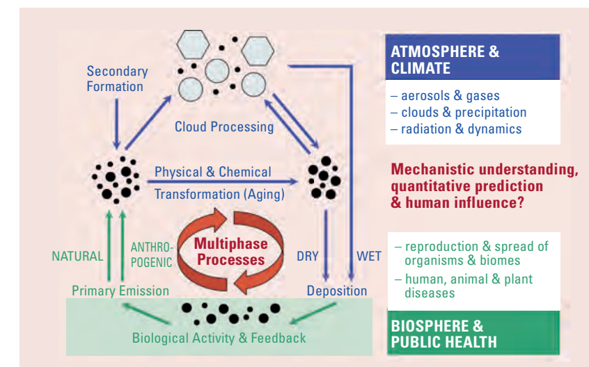
Figure 3: Atmosphere-biosphere exchange and multiphase processing of atmospheric particles and gases (adapted from Pöschl 2005 & 2011).
