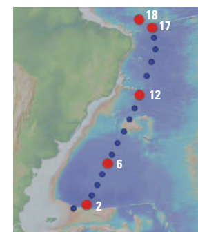
Figure 2: Cd isotope profiles (right) in the SW Atlantic from Geotraces cruise JC057 and stations (left).
