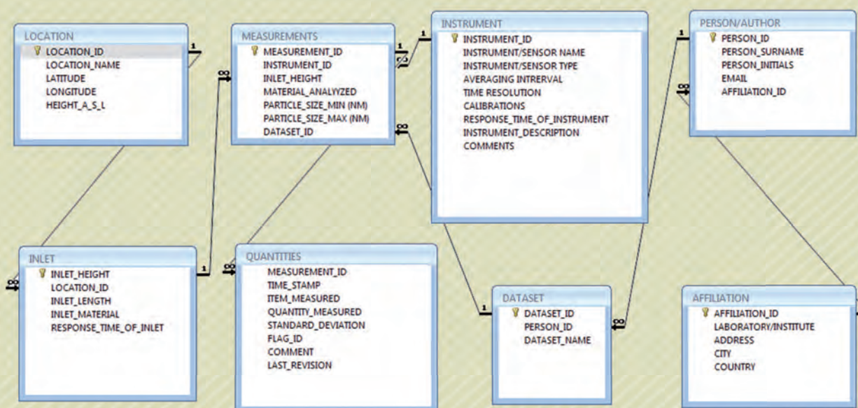
Figure 1: Structure of the ATTO database showing the respective columns and relationships.
